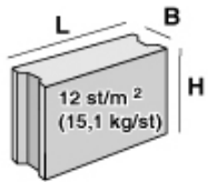
BIA 10-24 klinker LxBxH = 325x100x240 (9,0 ltr specie per m 2 )
